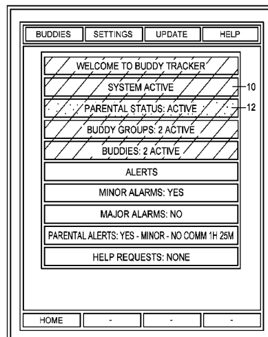
OPENING SCREEN
