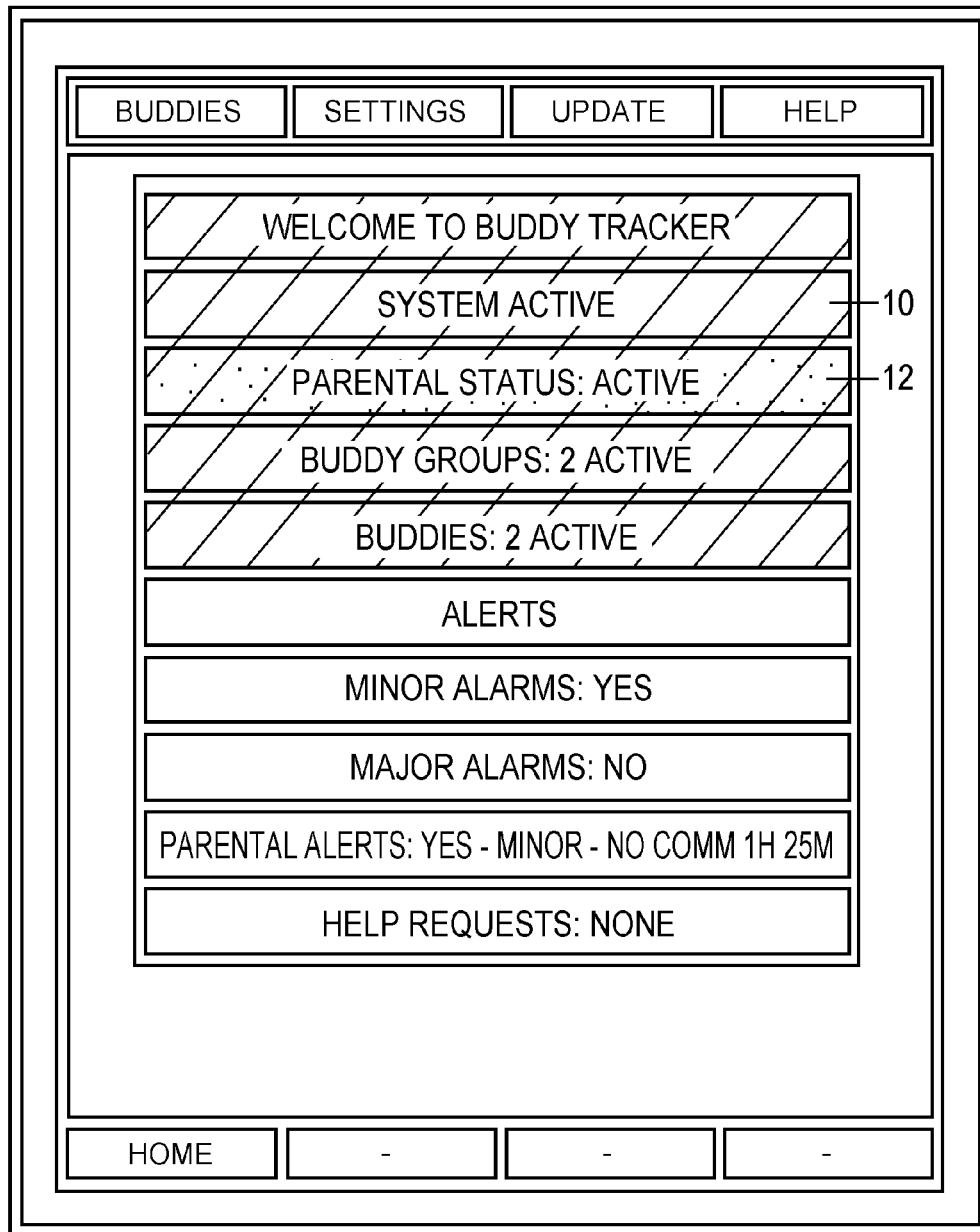
OPENING SCREEN
